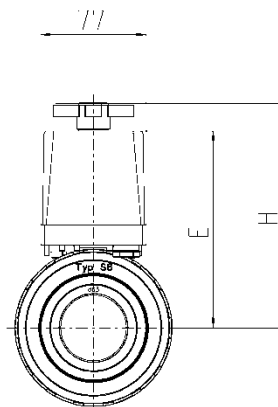
PVC ball valve DN32 – DN50 S6 E0510 ECO 230V
