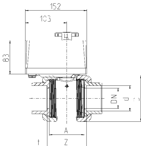
PVC ball valve DN32 – DN50 S6 E0510 ECO 230V
